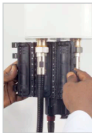
Jumperto-Antenna Application
