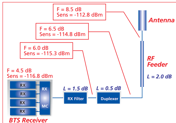
Figure 3a Sensitivity Improvement without TMA
