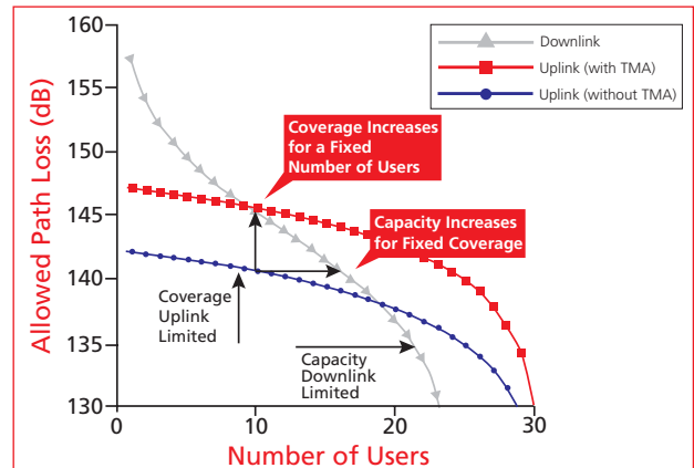
Figure 2 "Downlink Limited" Case
