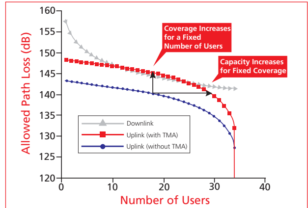
Figure 1 "Uplink Limited" Case
