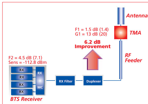
Figure 3b Sensitivity Improvement with TMA
