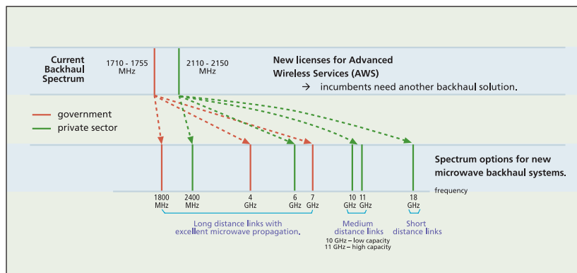
Figure 1 The backhaul relocation scenario caused by the AWS spectrum auctions
