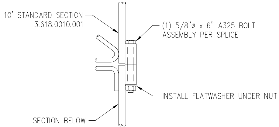
SPLICE DETAIL 1
